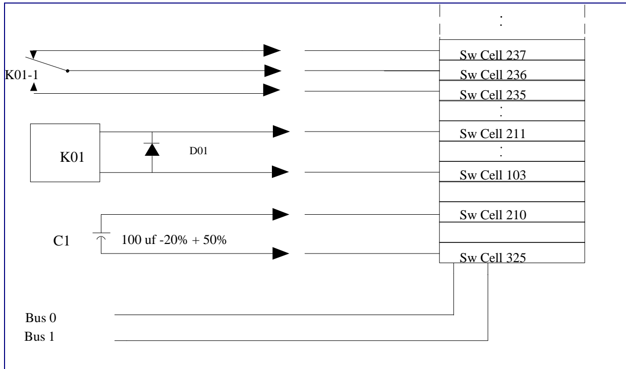
Figure 6. Adapted test circuit
