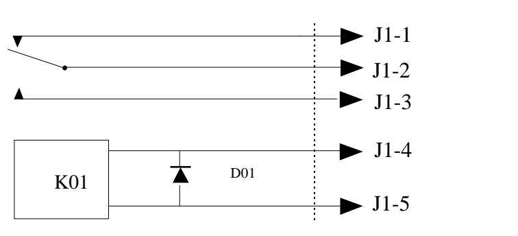
Figure 3. Relay circuit
