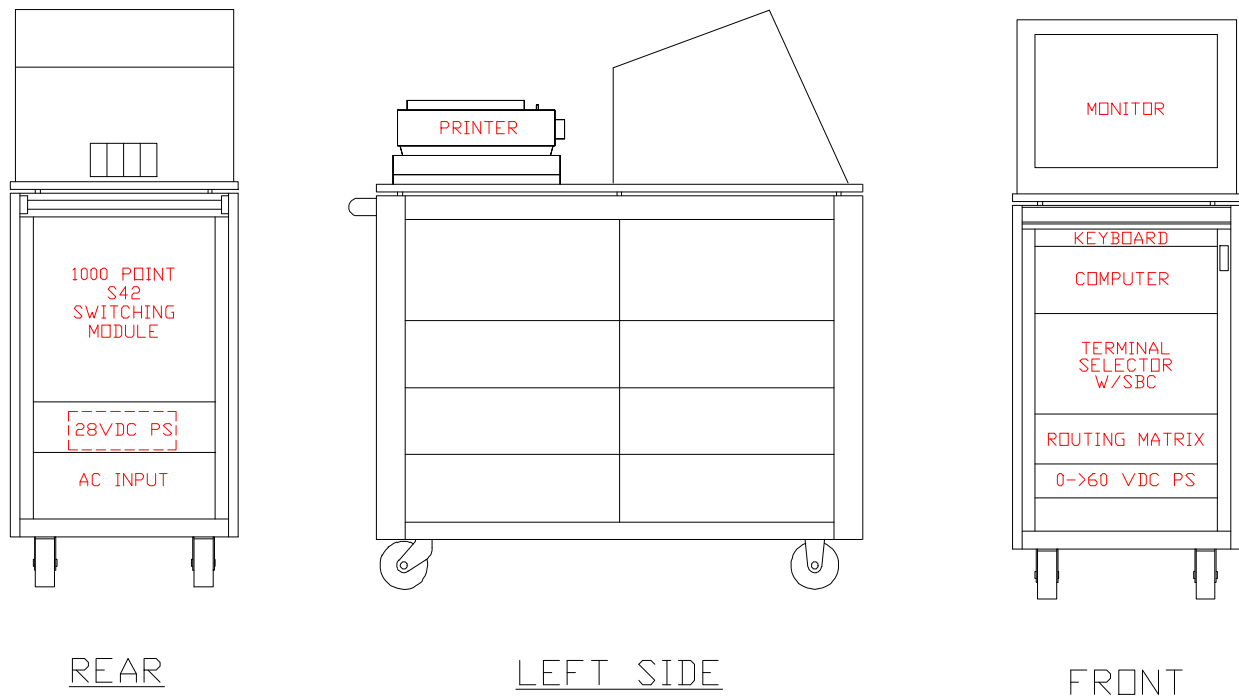
Figure 5. Portable 1,000-point, four-bus MBA analyzer
