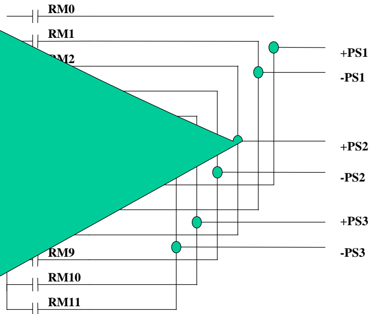
Figure 2. Typical bus to power connection—two buses to three power supplies
